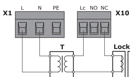
Figure 22. Connection diagram for an electromagnetic lock
