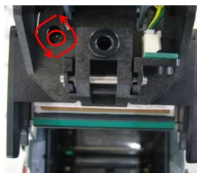
Figure 97 Print head angle
