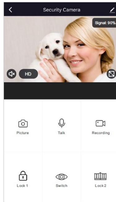
iOS System
