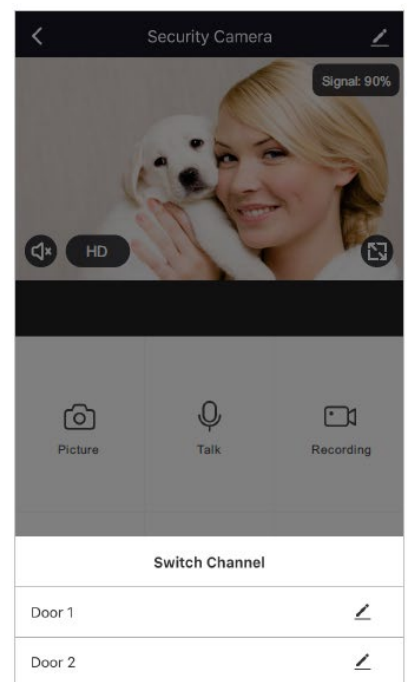
iOS System
