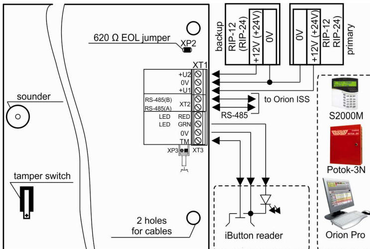
Figure 3. Module's Connection Diagram
