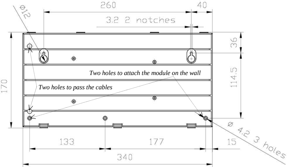
Figure 1. View and Overall and Mounting Dimensions of the Potok-BKI Module
