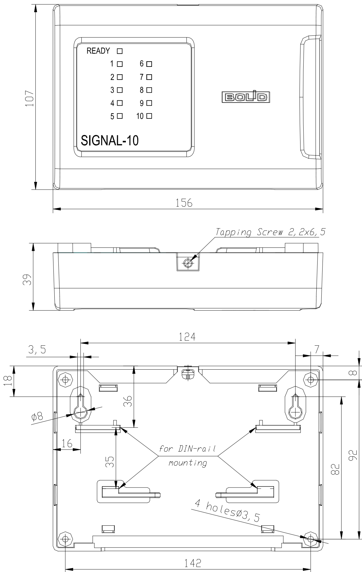
Figure 2. Signal-10 Overall and Mounting Dimensions
