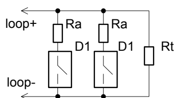
Figure 4. Detectors into a Fire Loop of the Type 1 Connecting Diagram
