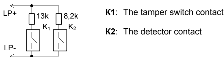
Figure 8. Wiring an Intruder Detector into Alarm Loops of the Type 5
