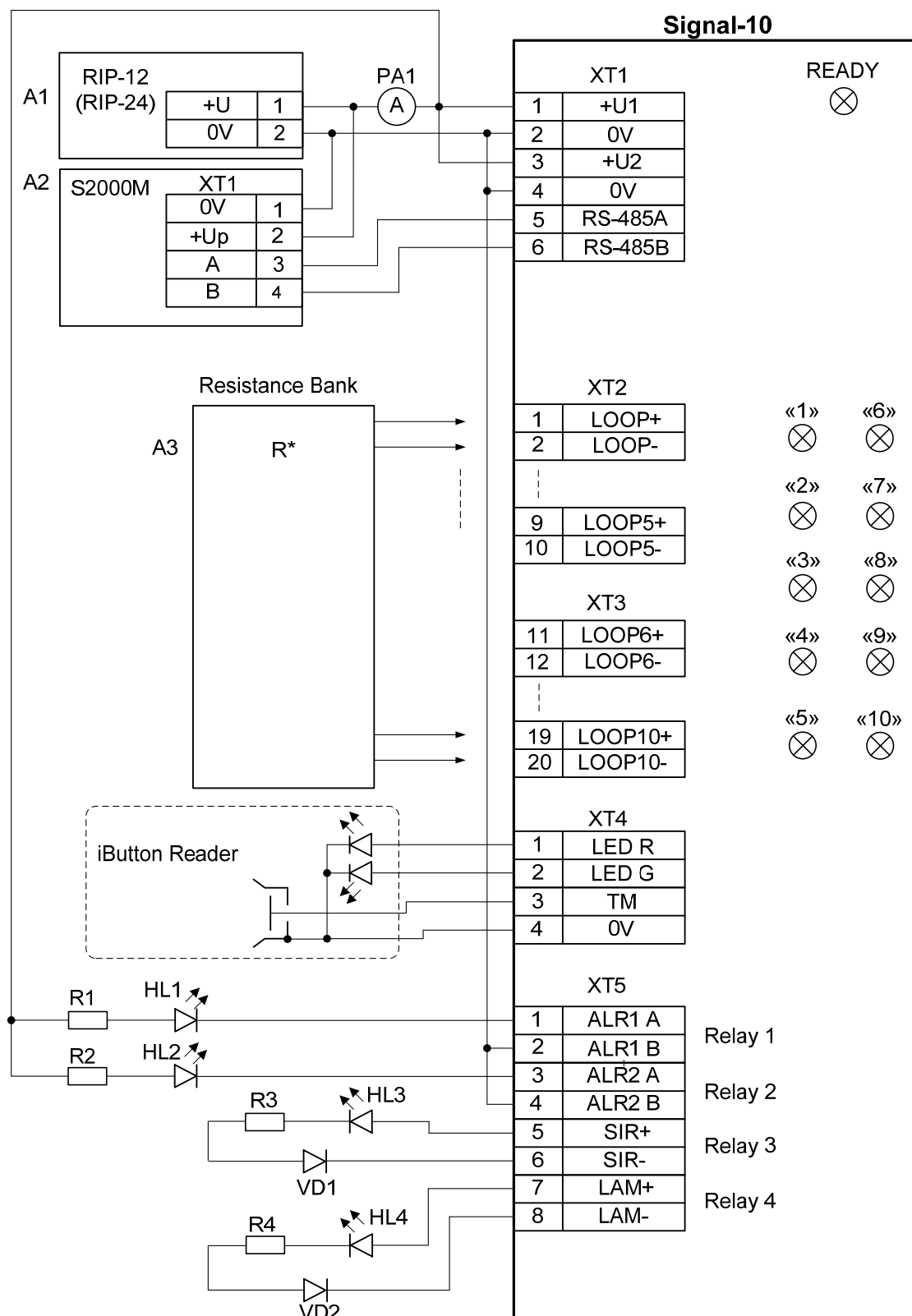
Figure 17. Wiring the Signal-10 for Operability Inspection
