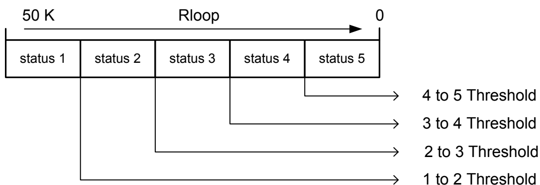
Figure 1. Thresholds of Transition between Different Statuses of Programmable Auxiliary Loops
