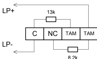
Figure 9. Wiring a Foton-SK Intruder Detector into Alarm Loops of the Type 5
