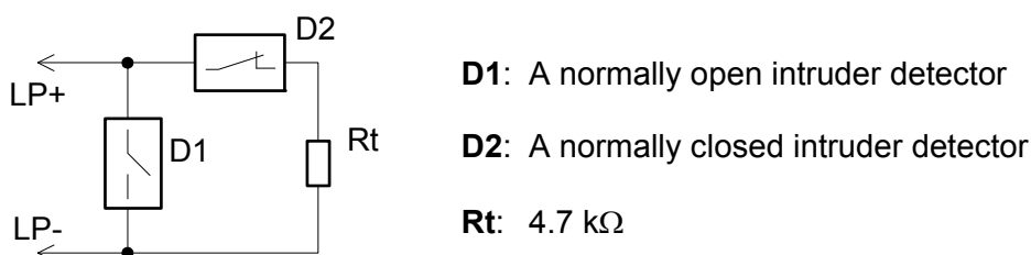
Figure 7. Wiring Intruder Detectors into Alarm Loops of the Type 4
