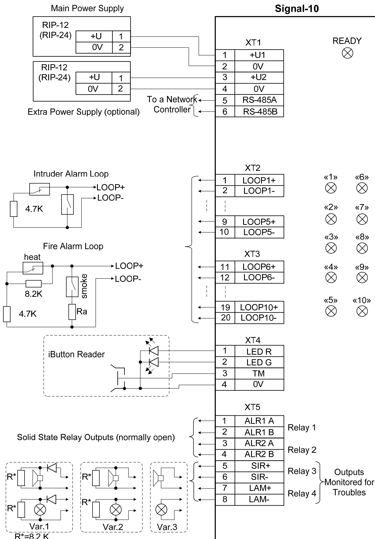
Figure 3. Signal-10 Connection Diagram
