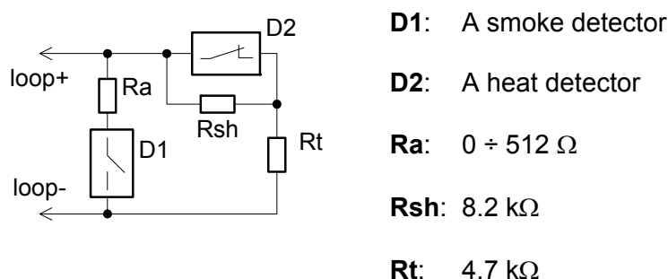
Figure 5. Smoke and Heat Detectors into a Fire Loop of the Type 2 Connecting Diagram
