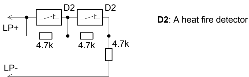
Figure 6. Heat Detectors into a Fire Loop of the Type 3 Connecting Diagram
