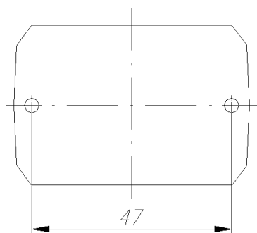
Figure 1. Drilling Pattern
