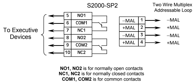
Figure 1 Connection Diagram
