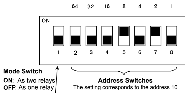
Figure 3 S2000-SP2 DIP-Switches
