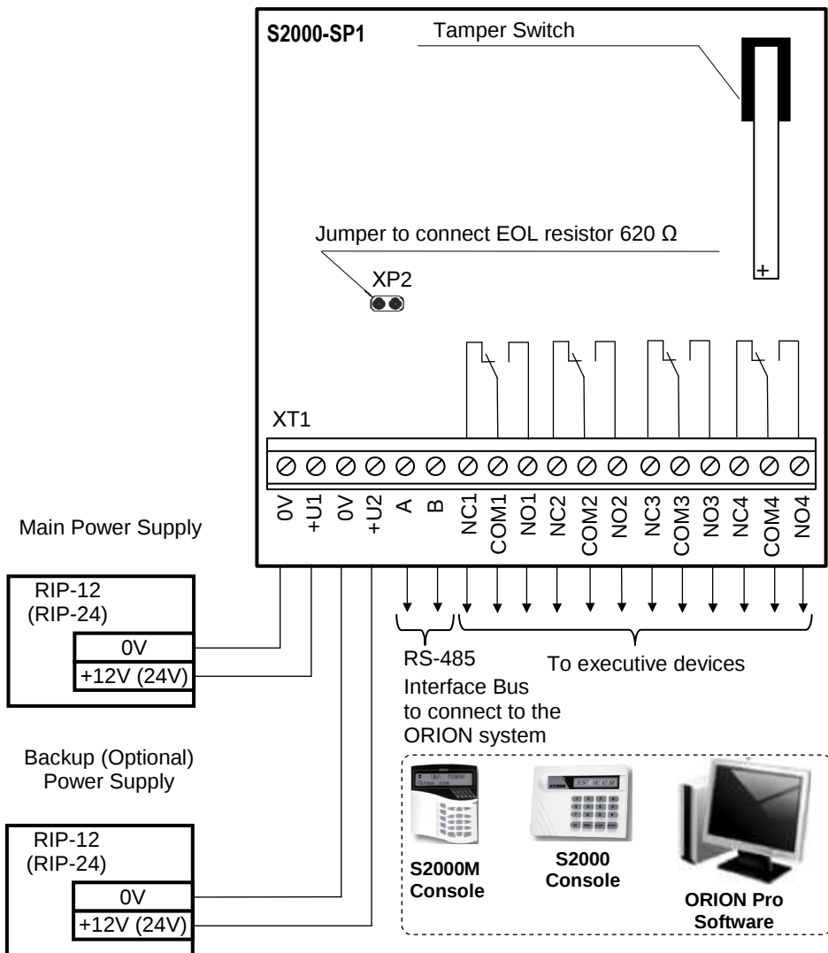
Figure 4. S2000-SP1 Wiring Diagram
