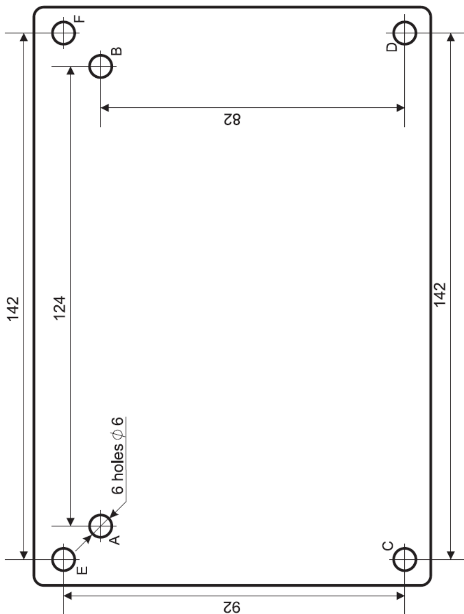
Figure 7. Mounting Pattern
