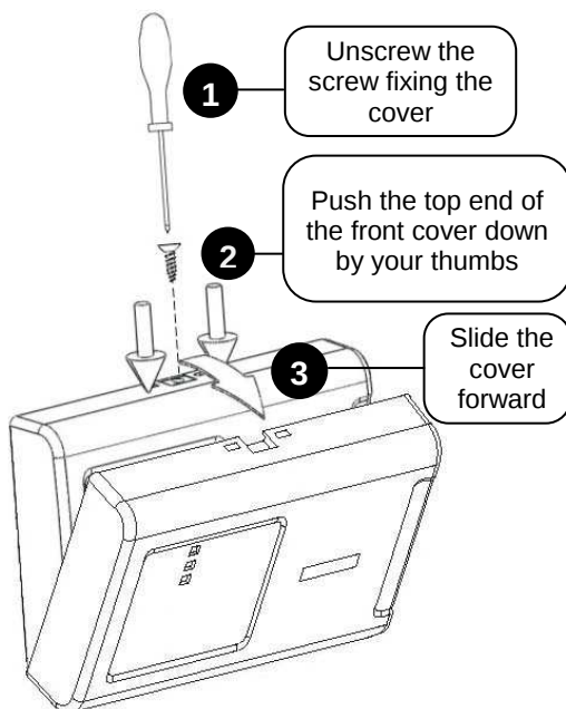
Figure 2. Opening the front cover
