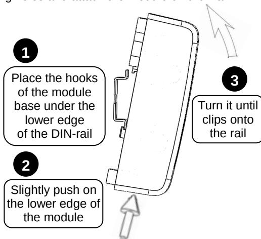
Figure 3. Installing the module on the DIN-rail
