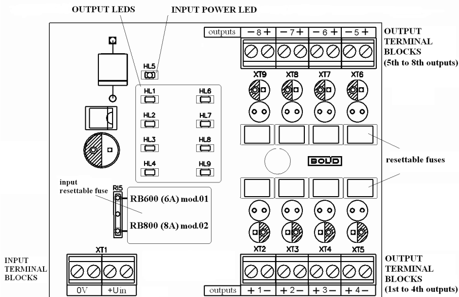
Figure 1. Terminal Blocks and LEDs
