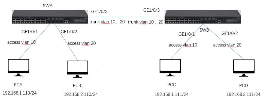
Figure 4-1 Network diagram
