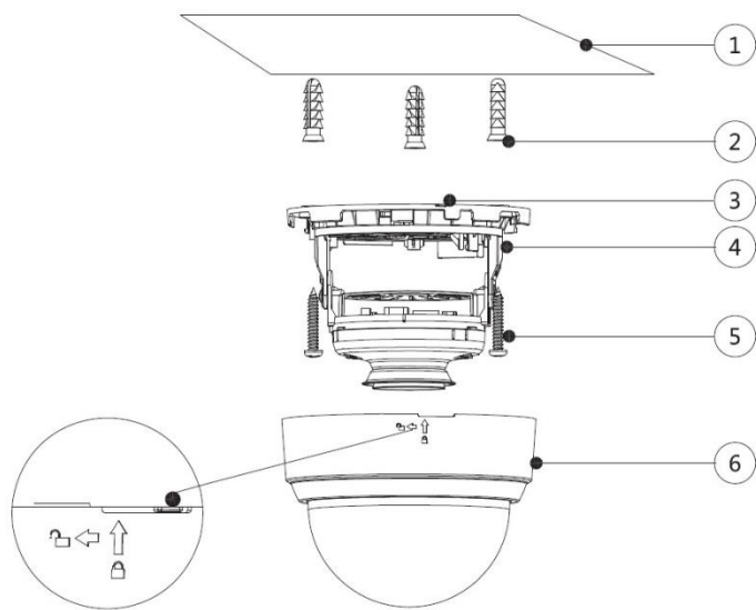
Figure 3-6 Model C installation
