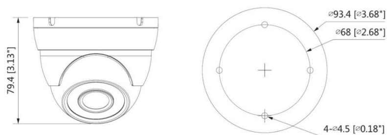
Figure 2-4 Model D (mm [in.])
