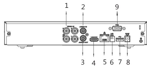
DHI-XVR4108HS-S2
