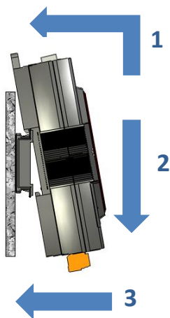
Mounting on a DIN-Rail
