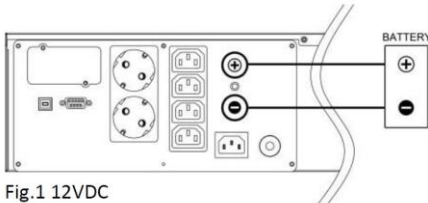
Fig.1 12VDC
