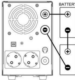
Fig.2 24VDC
