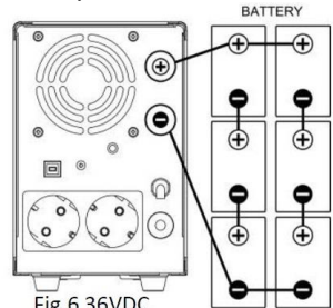
Fig.6 36VDC
