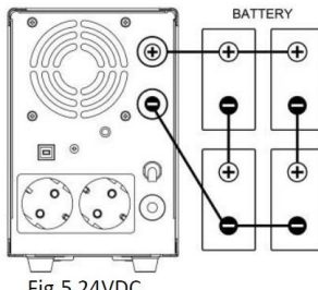
Fig.5 24VDC
