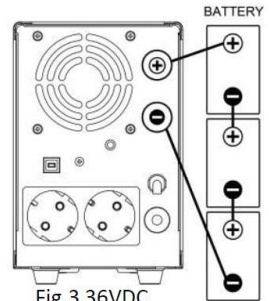
Fig.3 36VDC
