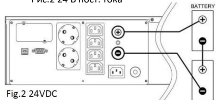
Fig.2 24VDC
