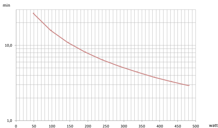
Figure 5. Runtime Graph INFOPDU800 / INFOPDU800PL / INFOPDU800LCD
