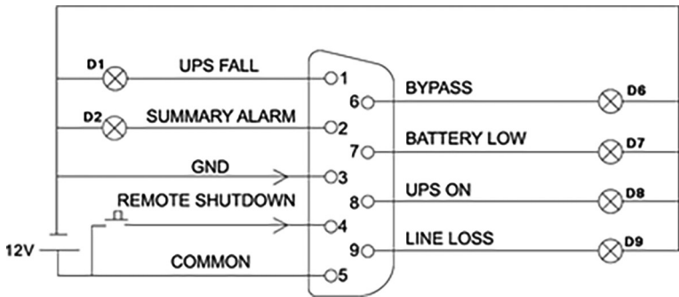
Figure 11. UPS status via DB-9 connector
