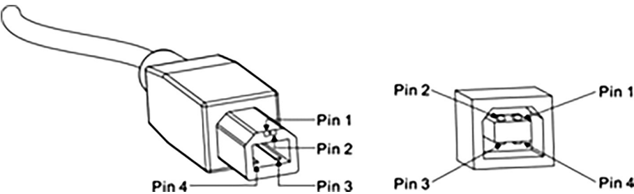
Figure 8. USB port
