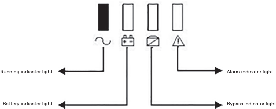
Figure 13. LED description
