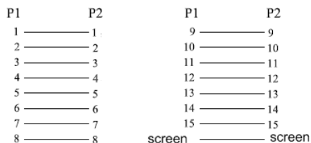
P1 HDB15M
