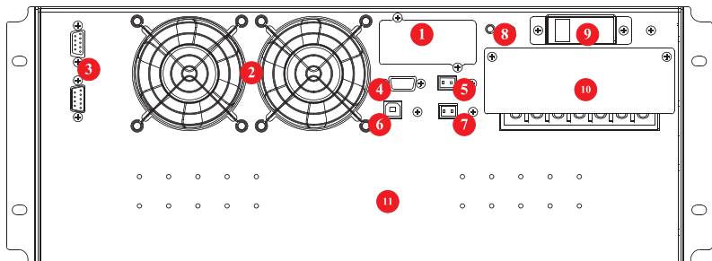
SW900G4-RTB-6/10 кВА (1:1)
