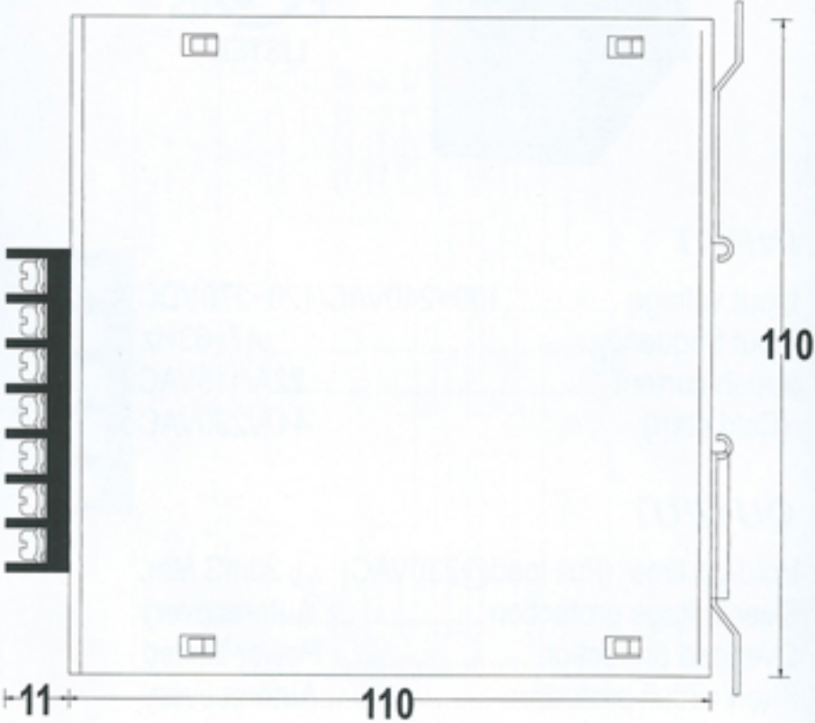
Dimensions:121(D)x110(H)x56(W)mm
