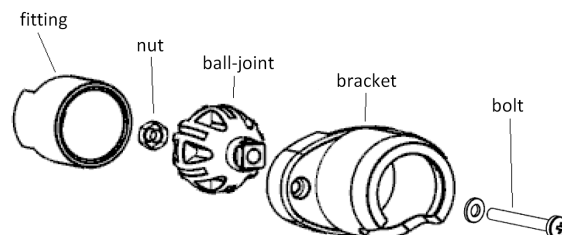
Figure 3: Mount Bracket Structure
