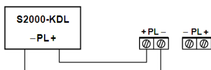
Figure 4. Connection Terminals
