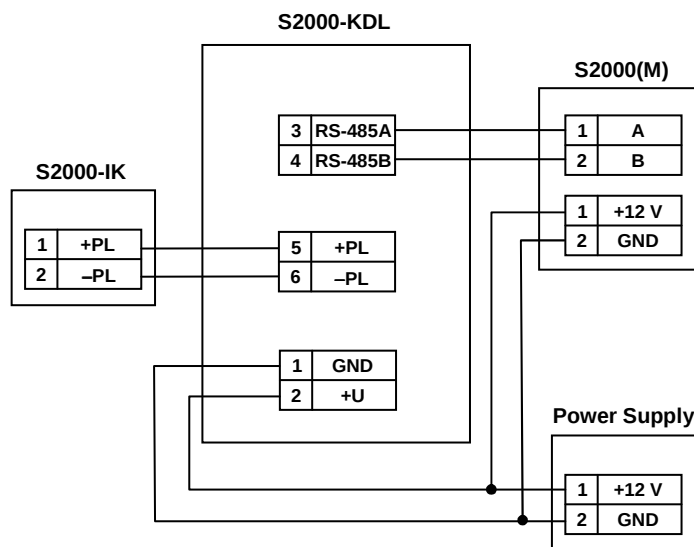
Figure 5. Connecting the Detector for Testing and Operation
