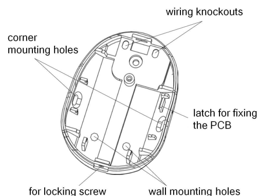
Figure 2: Rear Housing of the Detector
