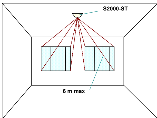
Figure 2: Ceiling Mounting
