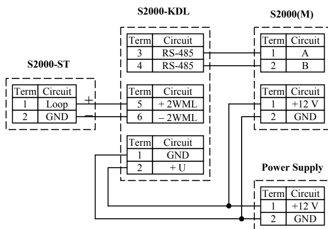
Figure 1: S2000-ST Detector Wiring Diagram
