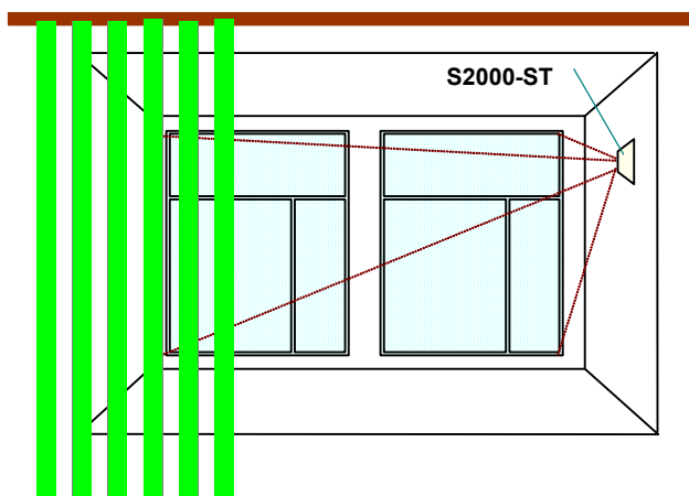
Figure 6: Mounting Behind a Window Covering
