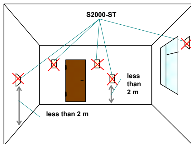
Figure 7: Inadvisable Mounting Location
