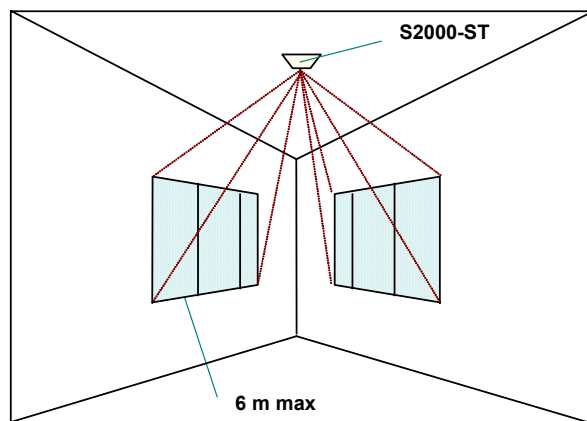
Figure 3: Ceiling Mounting
