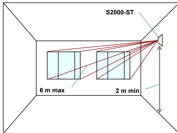
Figure 5: Adjacent Wall Mounting
