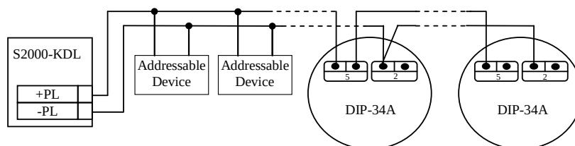
Figure 1. Connection Diagram
