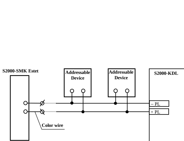
Figure 1: S2000-SMK Estet Wiring Diagram
