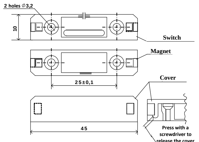
Figure 2: S2000-SMK Estet Mounting Dimensions
