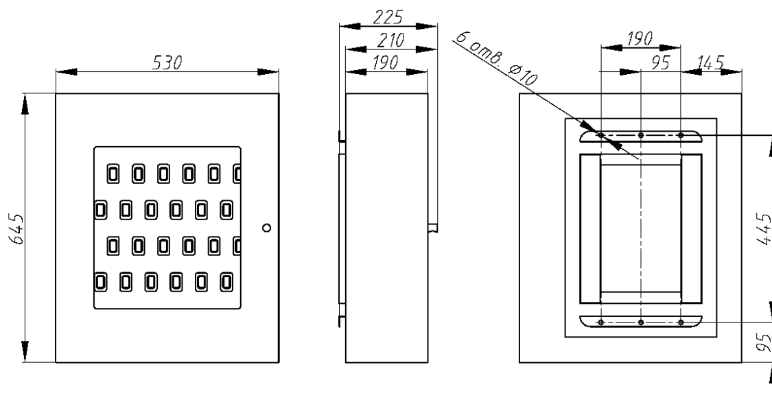
RusGuard KeyKeeper – 24 (аналогично для RusGuard KeyKeeper – 48)
