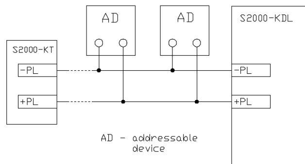
Figure 1 Wiring Diagram
