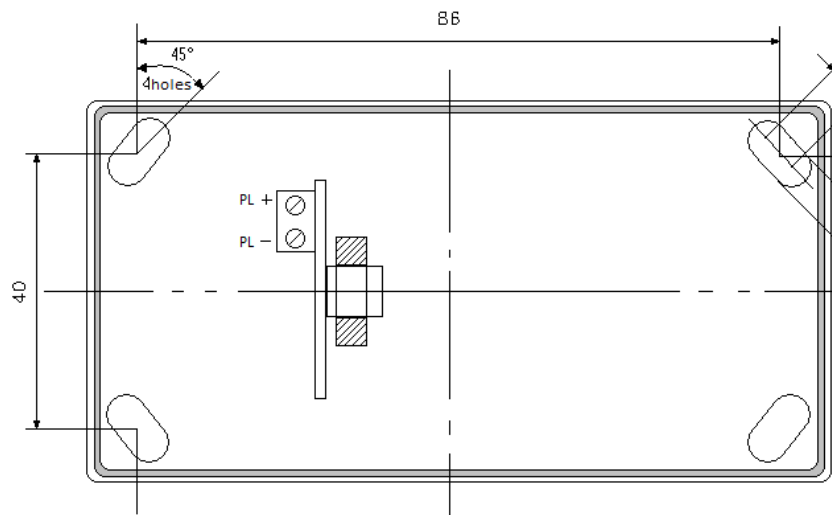
Figure 2 Mounting Dimensions
