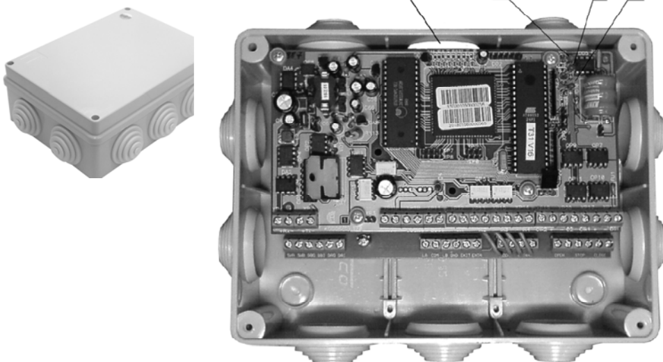
Figure 1 – Access controller (front) and view of the Controller with Body Cover Removed
