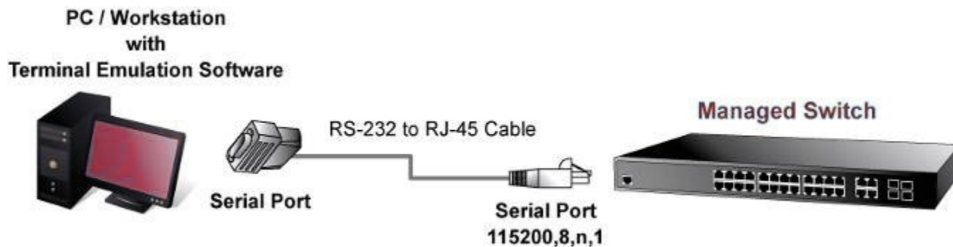
Figure 3-1: Console Management
