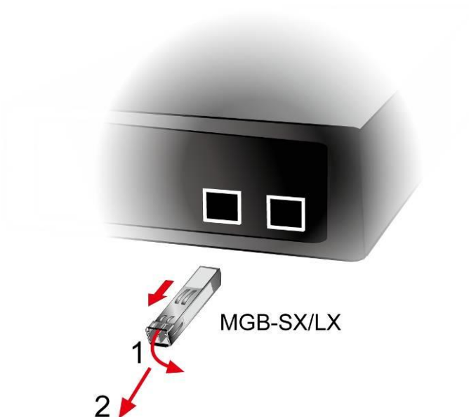
Figure 2-2-2 How to Pull Out the SFP Transceiver
