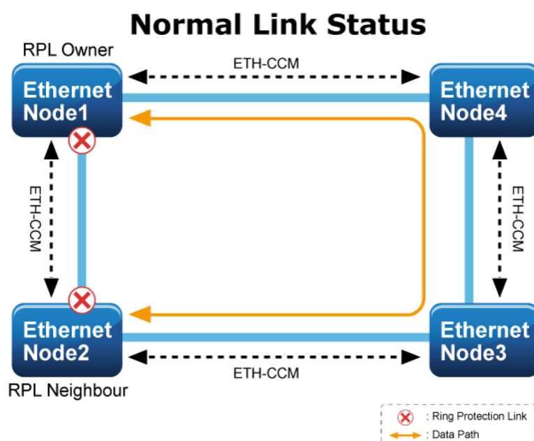
Figure 4-6-1-1 Ring Mode
