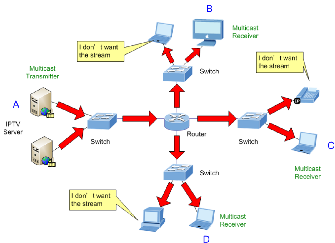
Figure 4-3-79 Multicast Flooding
