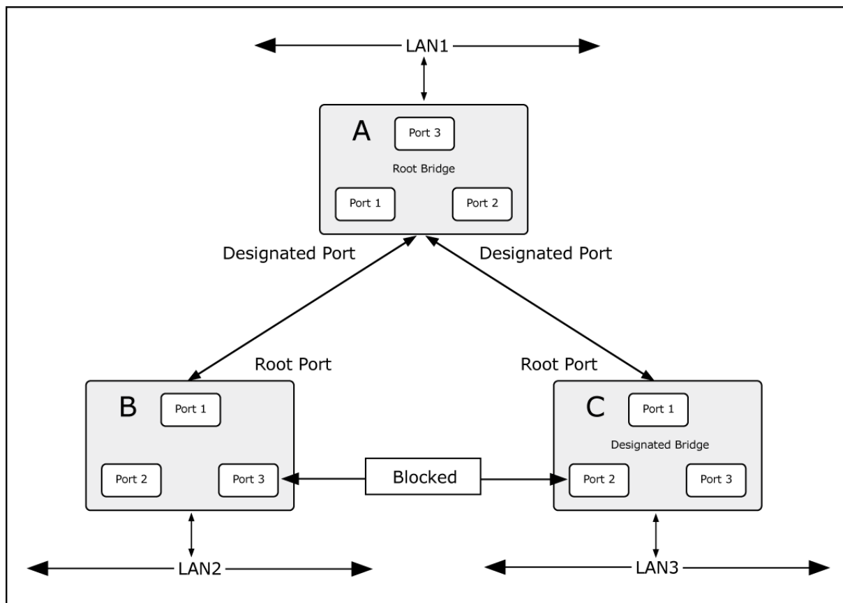
Figure 4-3-58 After Applying the STA Rules
