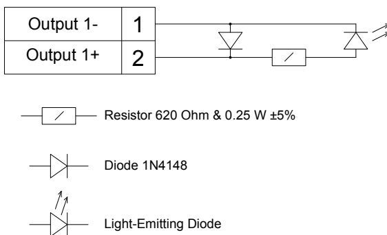
Figure 6. The Schematic of a Discharge Circuit Simulator
