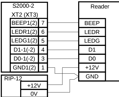
Figure 12. Schematic for Connecting Readers with Wiegand or ABA Track-II Interface
