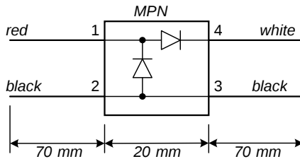
Figure 1. The Schematic and the View of the MPN
