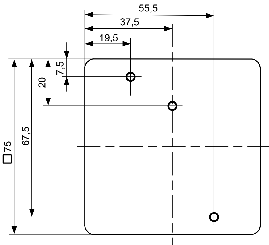
Figure 1 (Drilling pattern, scale 1:1)
