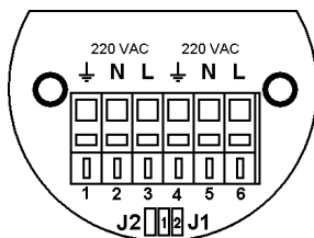
б) BC-07e-Ex-3(I)-230VAC
