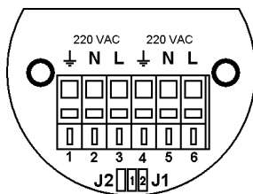
б) BC-07e-O-3(I)-230VAC
