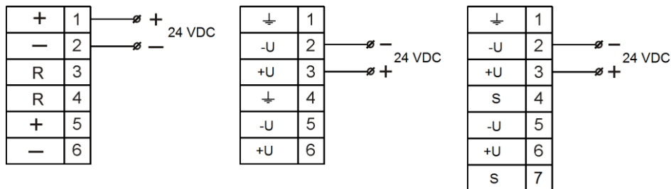
а) BC-07e-O-3(И)-24VDC
