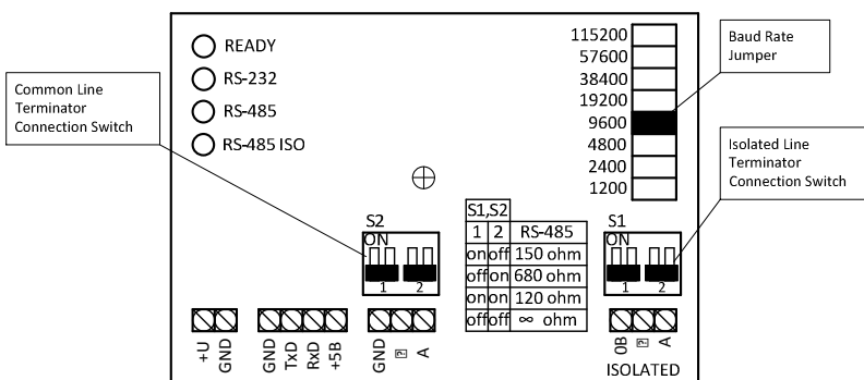
Figure 4: S2000-PI Layout
