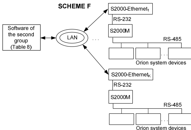
Figure 3. Common Diagrams for Using the S2000-Ethernet as a Component of an Orion System
