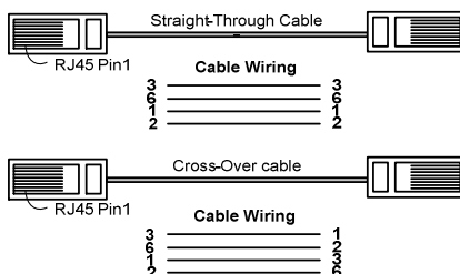
Figure 7. Types of Ethernet Cables
