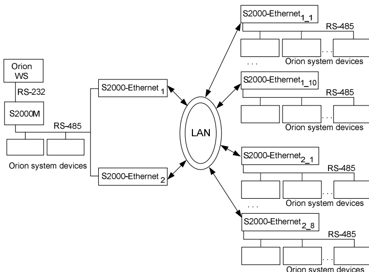
Figure 5. An Example of Connection Diagram for the S2000-Ethernet
