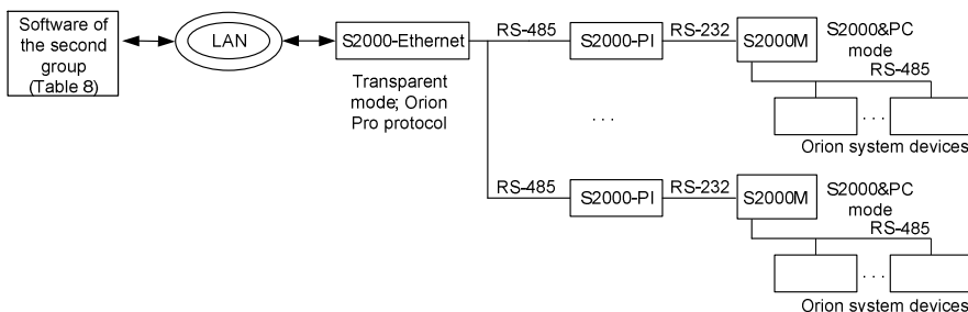
Figure 4. Diagram for Connection of Several S2000M Consoles to a Single Virtual COM Port
