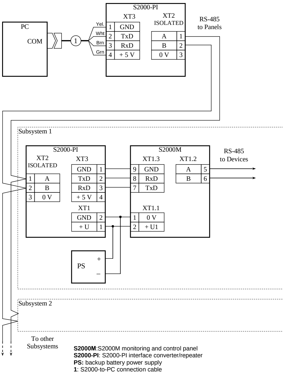
Figure 8. Multiple S2000M Connection to Orion Pro Workstation
