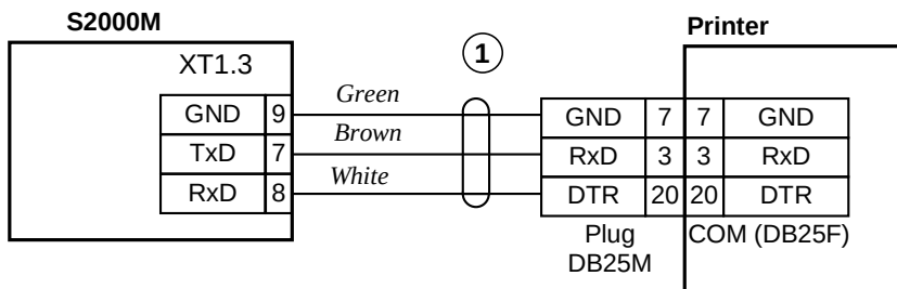
Figure 7. Connection of Printer to S2000M
