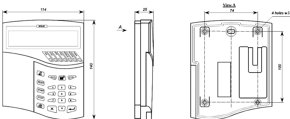
Figure 1. Dimensions and Installation Layout
