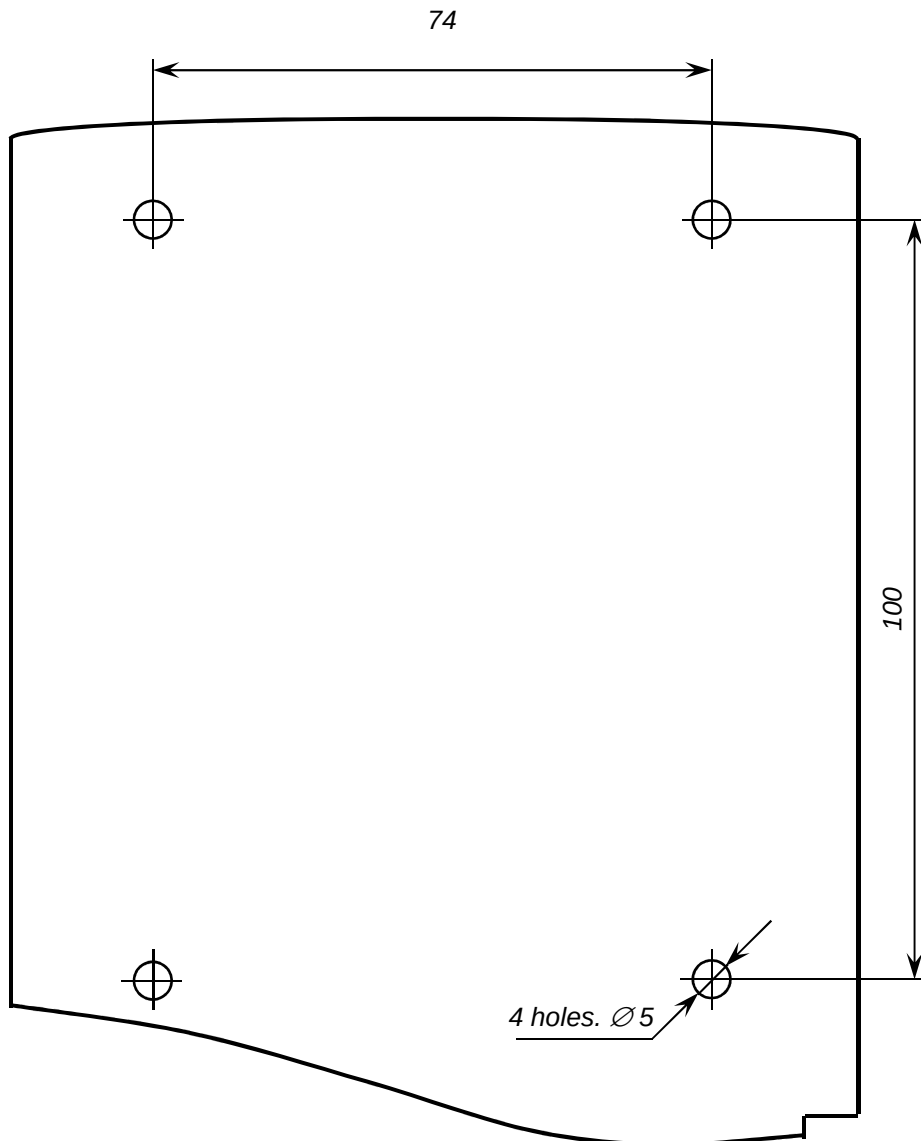
Figure 13. Drilling Pattern
