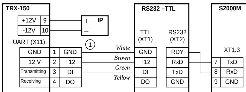
Figure 9. ATS100 Connection to S2000M
