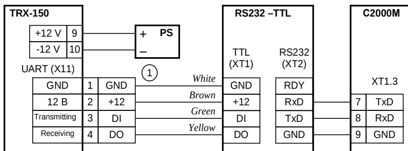
Figure 10. TRX-150 Connection to S2000M for Transmission to Orion-Radio
