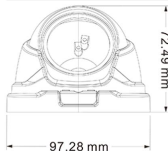
PVC-IP4F (DF2.8A, DF2.8PA)
