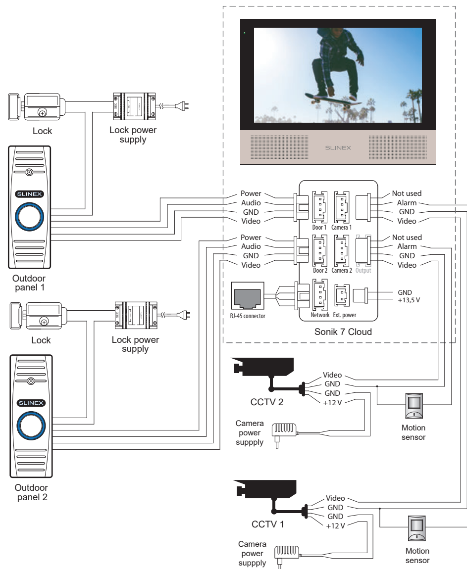
Diagram 1. Sonik 7 Cloud outdoor panels, cameras and locks connection.
