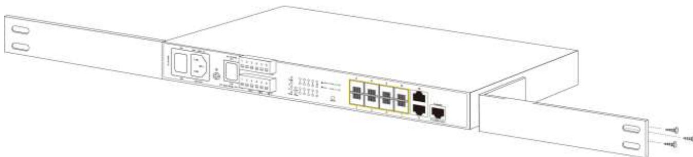
Figure 2-8: Attach Brackets to the Managed Metro Switch.
