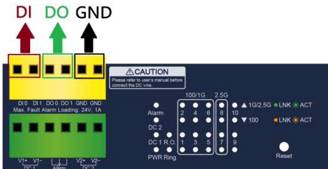
Figure 2-3: Wiring the Digital Input/Digital Output and Ground
