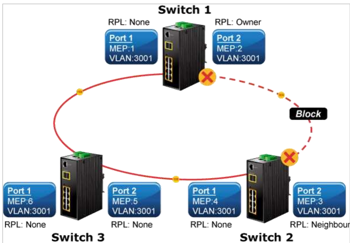
Figure 4-6-1-4: Ring Example Diagram
