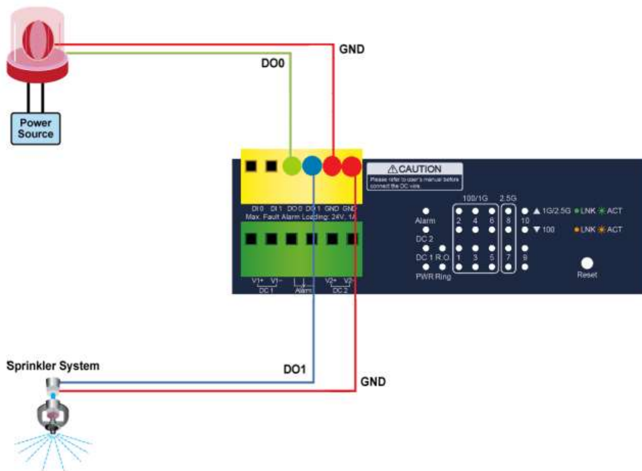
Figure 2-6: Wiring DO0 and DO1 to Open Detector
