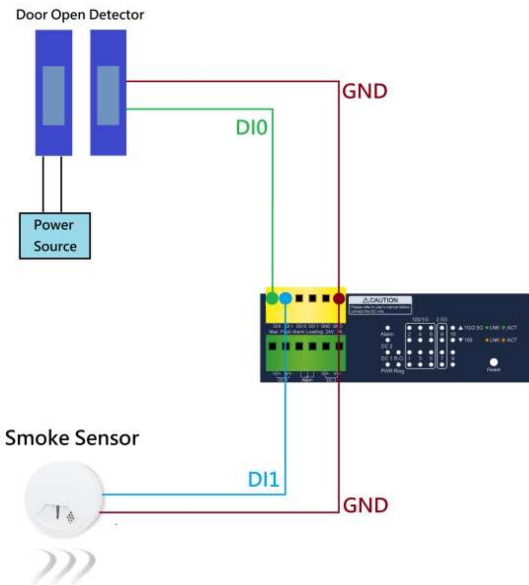
Figure 2-5: Wiring DI0 and DI1 to Open Detector
