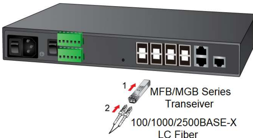
Figure 2-10: Plugging in the SFP Transceiver
