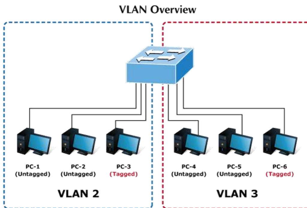
Figure 4-3-3-7: Two Separate VLANs Diagram
