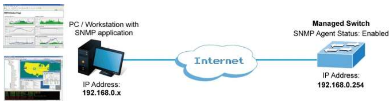
Figure 3-4: SNMP Management
