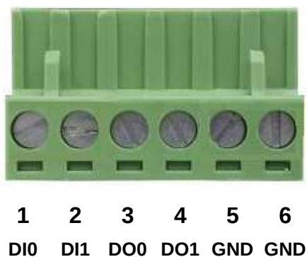
Figure 2-4: 6-pin Terminal Block for DI and DO Wiring Input
