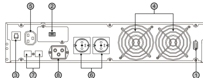
RT-3K-LCD
