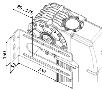
TR-10024-400/TR-13018-400
