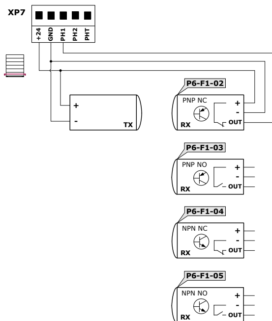
Photocells with transistor output of different type
