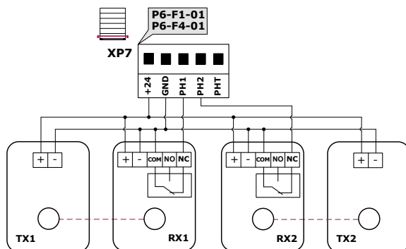
Two pairs of wired photocells
