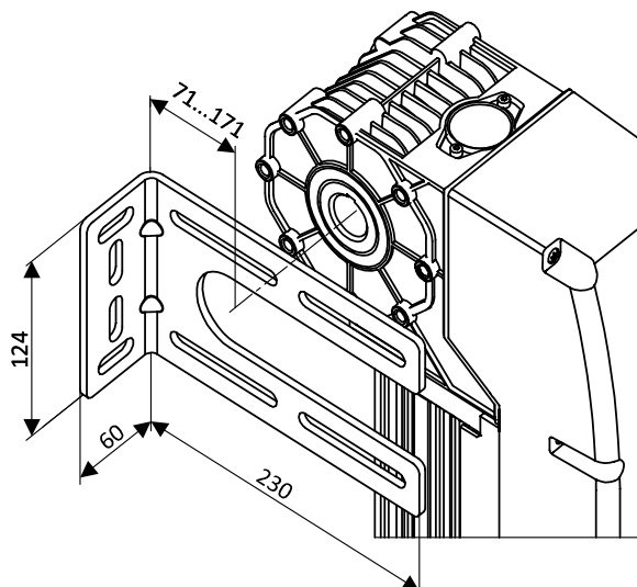
Figure 3. Dimensions of the mounting bracket
