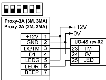
Figure 7. Reader Connection Diagrams
