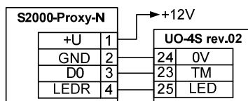
Figure 7. Reader Connection Diagrams
