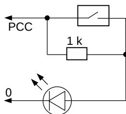
Patrol Check Circuit
