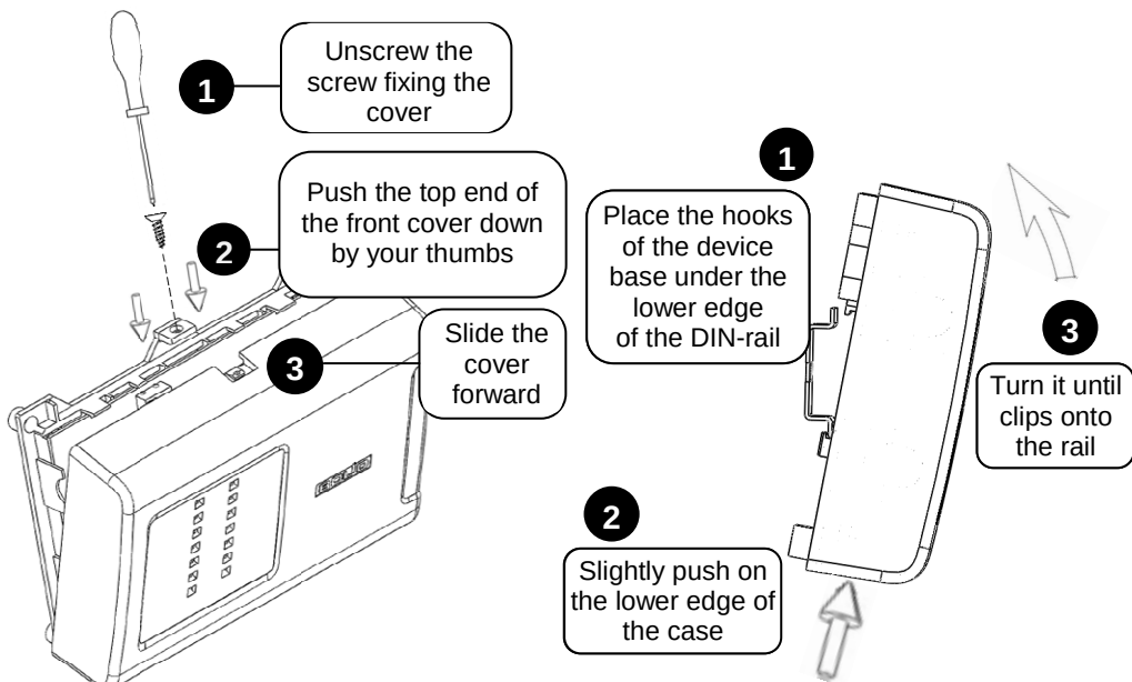
Figure 2. How to Remove the Cover
